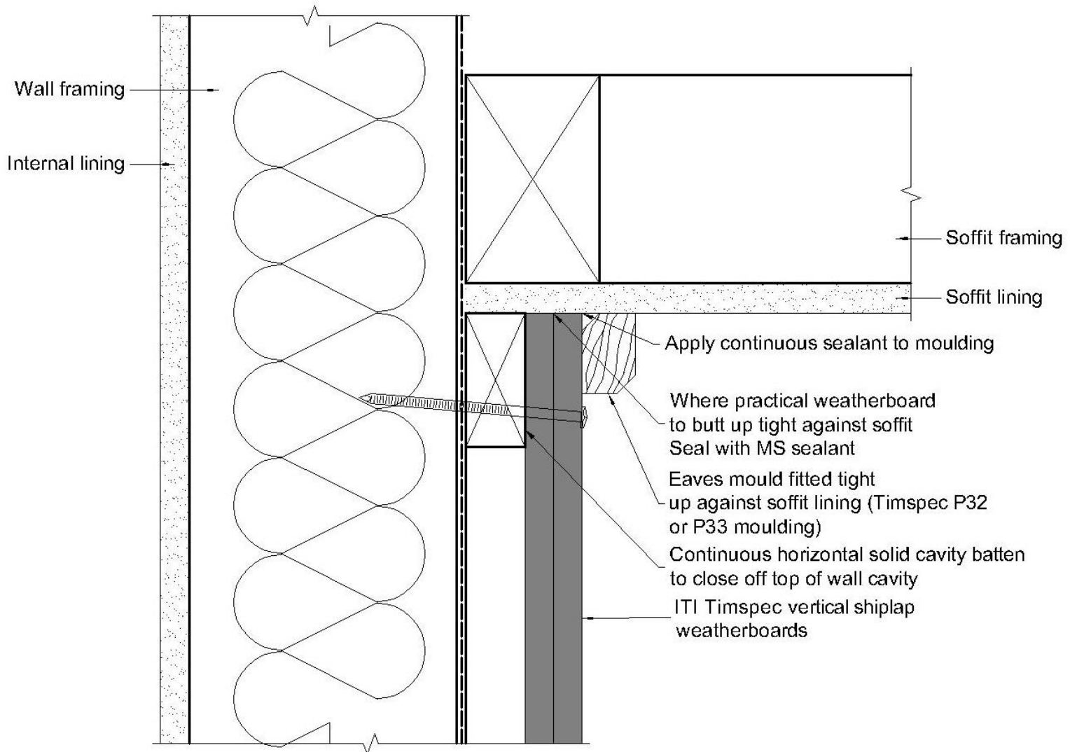
VC 601 Roof/ Wall Top Plate – Flat Soffit
