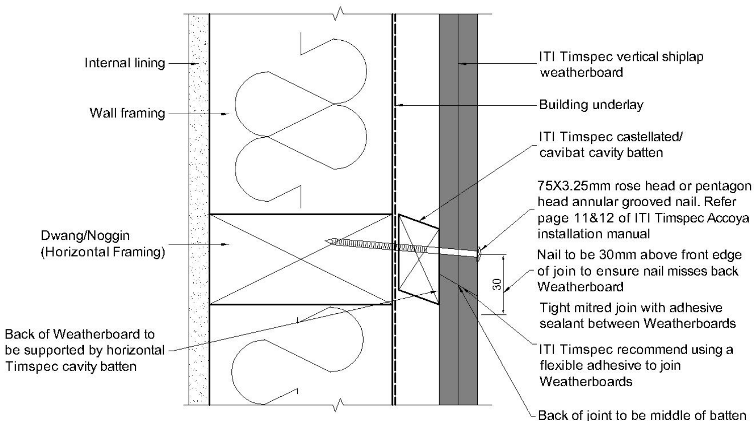
VC 402 Within Board Joint – Scarf Joint
