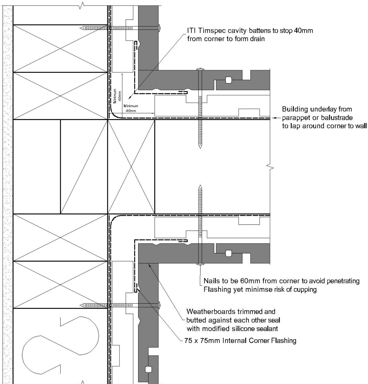
VC 702 Balustrade, Intersection with Wall
