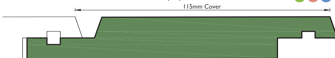
P51 Bevel Grooved Vertical Shiplap Profile
